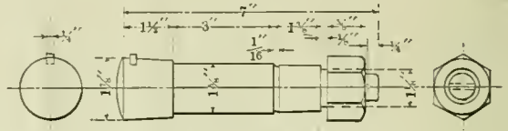
TOP PINS IN COMBINATION LEVER
